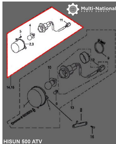
HISUN 500 ATV
